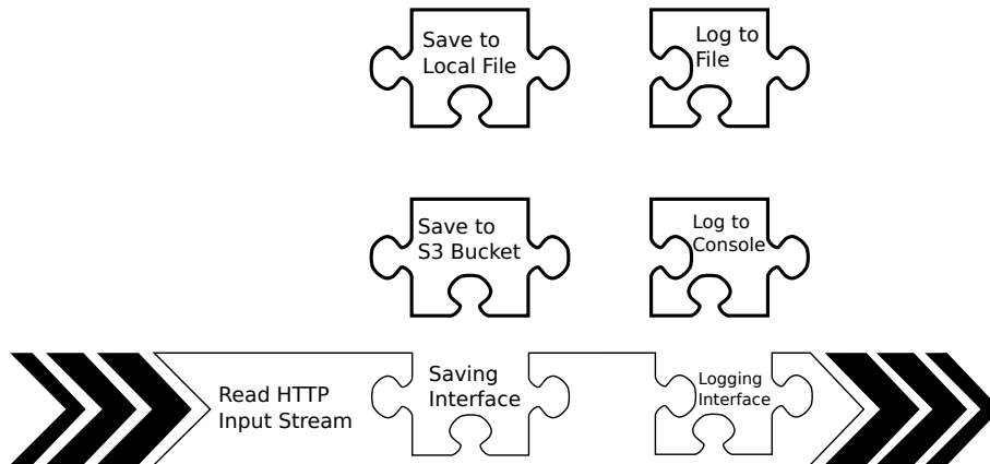
Figure 308: Using Interfaces and DI to build a flexible file upload
